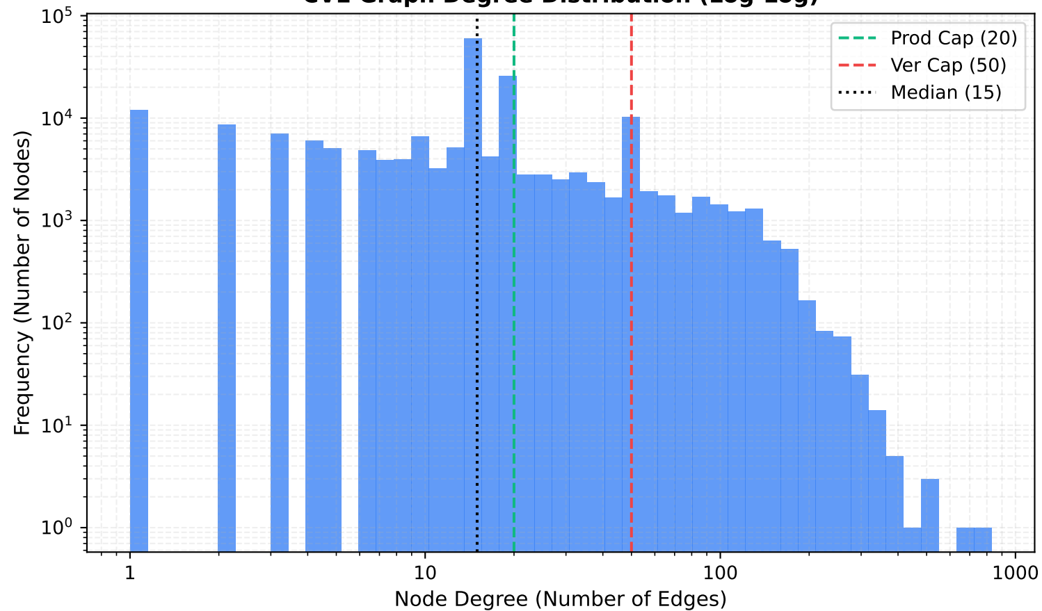
CVE Graph Degree Distribution (Log-Log)
